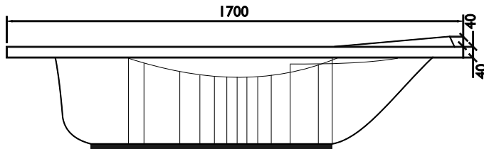
SIDE ELEVATION
