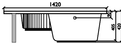
SIDE ELEVATION
